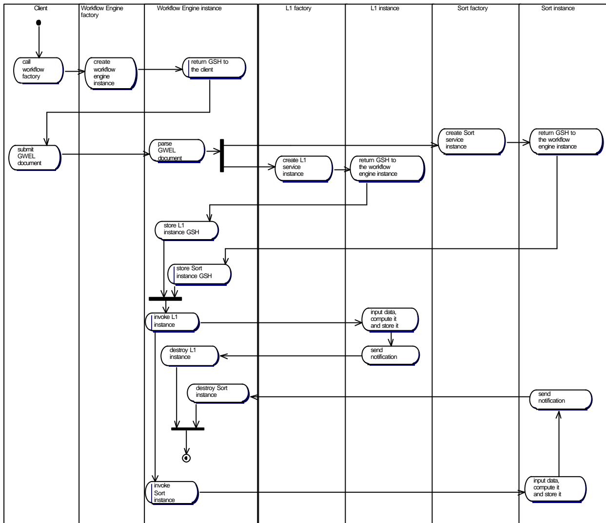
Figure 6 - Activity diagram
